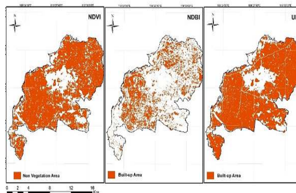
Figure 3. Spatial distribution of the built-up area of the remote sensing index in 2017
