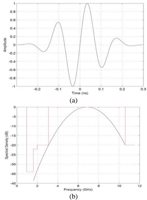
Figure 5. (a) A modulated Gaussian pulse and (b) its spectral density which fits into the FCC spectral mask for handheld systems.
