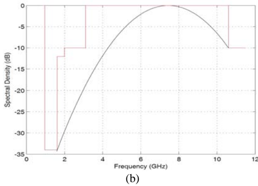
Figure 4. (a) A modulated Gaussian pulse and (b) its spectral density which fits into the FCC spectral mask for indoor systems
