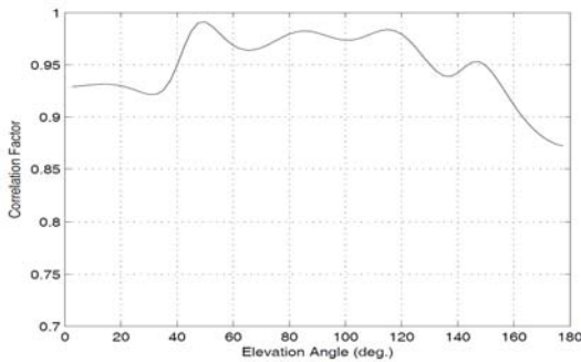
Figure 15. Correlation factor for the second optimized antenna as a function of elevation angle
