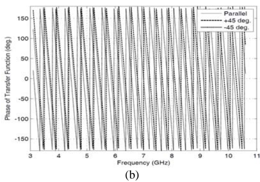
Figure 30. Transfer Functions of two-antenna systems. (a) Magnitude and (b) phase (calculated for the third optimized antenna)
