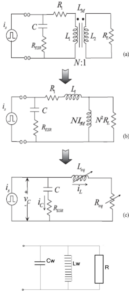
Figure 3. (a) Based circuit of the induction heater. (b) Equivalent circuit of the induction heater on a transformer concept. (c, d) Simplified equivalent circuit of the induction heater.
