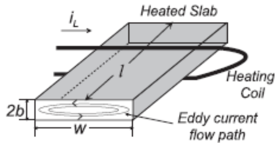
Figure 2. Model of slab for one turn coil.
