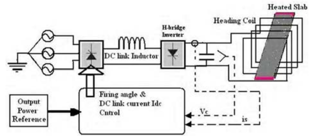
Figure 1. a) A model of Induction heater, b) Block diagram of induction heating system.
