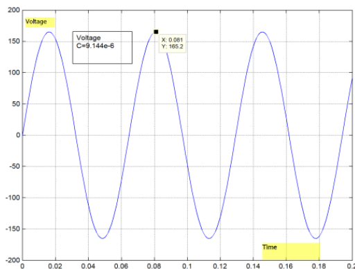
Figure 7- V_c voltage of capacitance with C=9.144e-6 .
