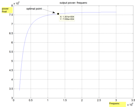
Figure 5- altering output power with frequency.
