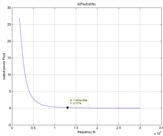
Figure 6- d(P_{out})/d(f_s) .
