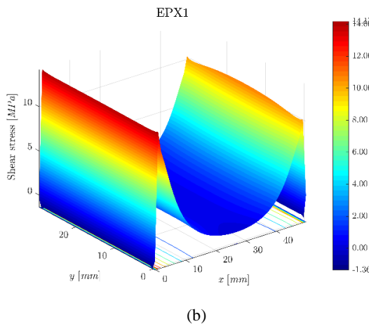
Figure 5. Peel and shear stress distribution for 10° tapering adherends angle configurations
