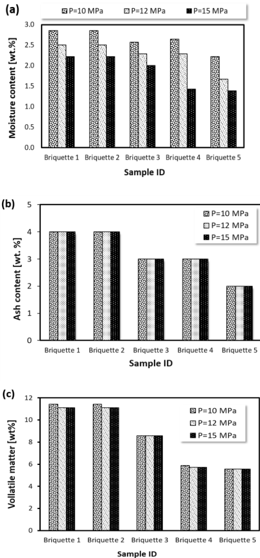
Figure 2. Effect of compaction pressure and mixing ratios on (a) moisture content, (b) ash content, and (c) volatile matter
