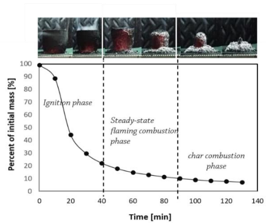
Figure 5. Normalized burning rate (NBR)
