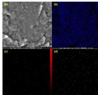
Figure 4. (a) SEM image of the nanocomposite modified CPE used for map analysis, disperse pattern of carbon (b), samarium (c), oxygen (d)
