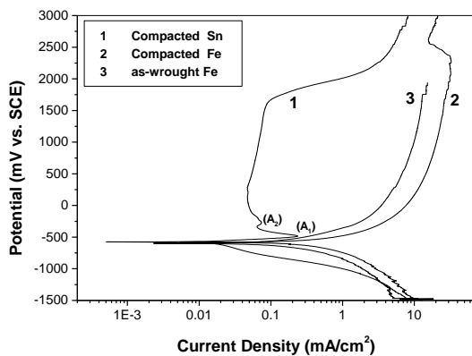
Figure 2. Potentiodynamic polarization curves of electrodes of compacted tin and iron powders compared with as-wrought iron in 0.1M \text{H}_3\text{PO}_4 solution.
