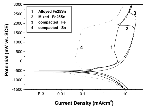
Figure 3. Potentiodynamic polarization curves of compacted powders of tin, iron, Fe-25at.% Sn admixture and Fe-25at.%Sn supersaturated solid solution in 0.1M \text{H}_3\text{PO}_4 solution.
