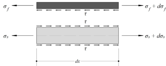
Figure 2. Free body diagram
