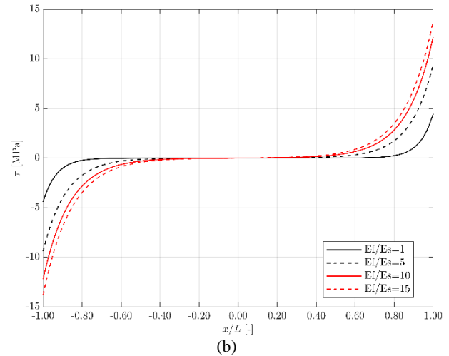
Figure 3. Effect of the Young moduli ratio of the adherents on the normal stress distribution in the reinforcement (a) and on the interfacial shear stress distribution (b)
