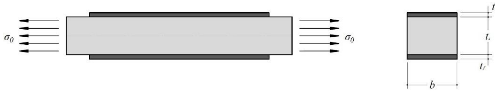
Figure 1. Reinforced structural element, longitudinal and cross-section
