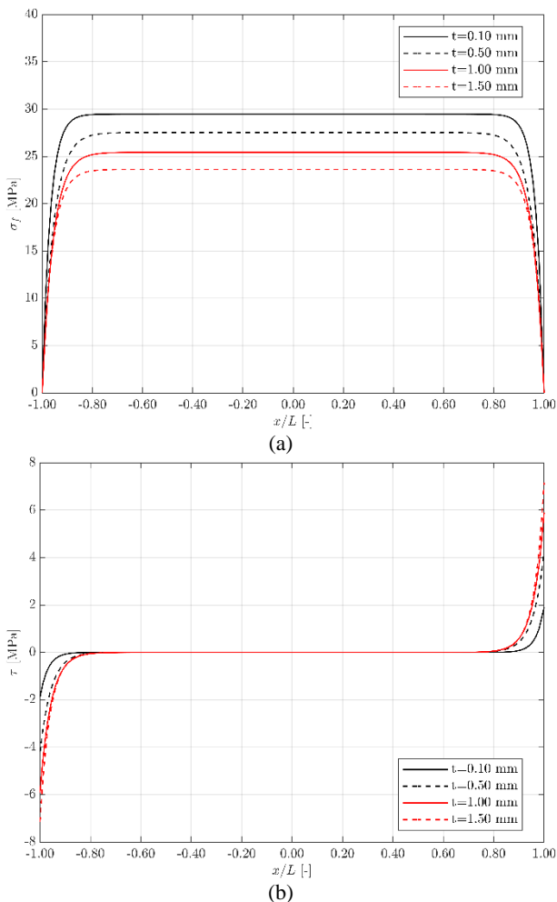
Figure 4. Effect of the reinforcement's thickness on the normal stress distribution in the reinforcement (a) and on the interfacial shear stress distribution (b)
