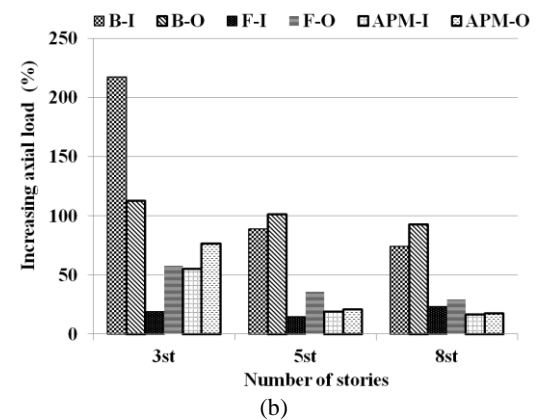
Figure 7. Increasing axial loads of the columns around the removal location compared to the non-removal mode a: buildings with CBs b: buildings with BRBs
