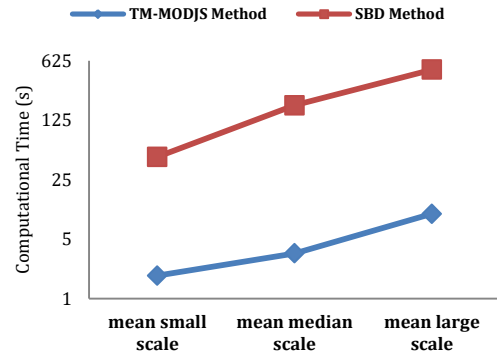
Figure 5. Comparing computational time for three scale
