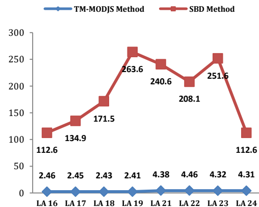
Figure 3. Comparing computational time for three methods in Medium scale problems
