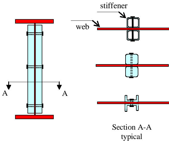
Figure 1. Typical bolted stiffeners.
