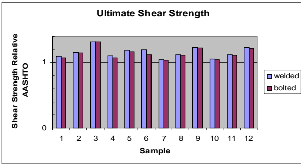
Figure 3. Shear strength - welded stiffener vs. rigid bolted stiffener.
