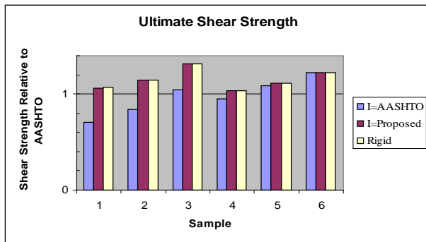
Figure 5. Shear strength of girders reinforced by bolted stiffeners.
