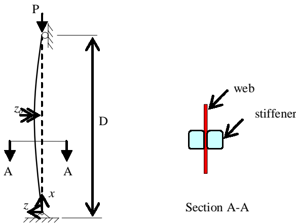
Figure 4. Idealized column - bolted stiffener.
